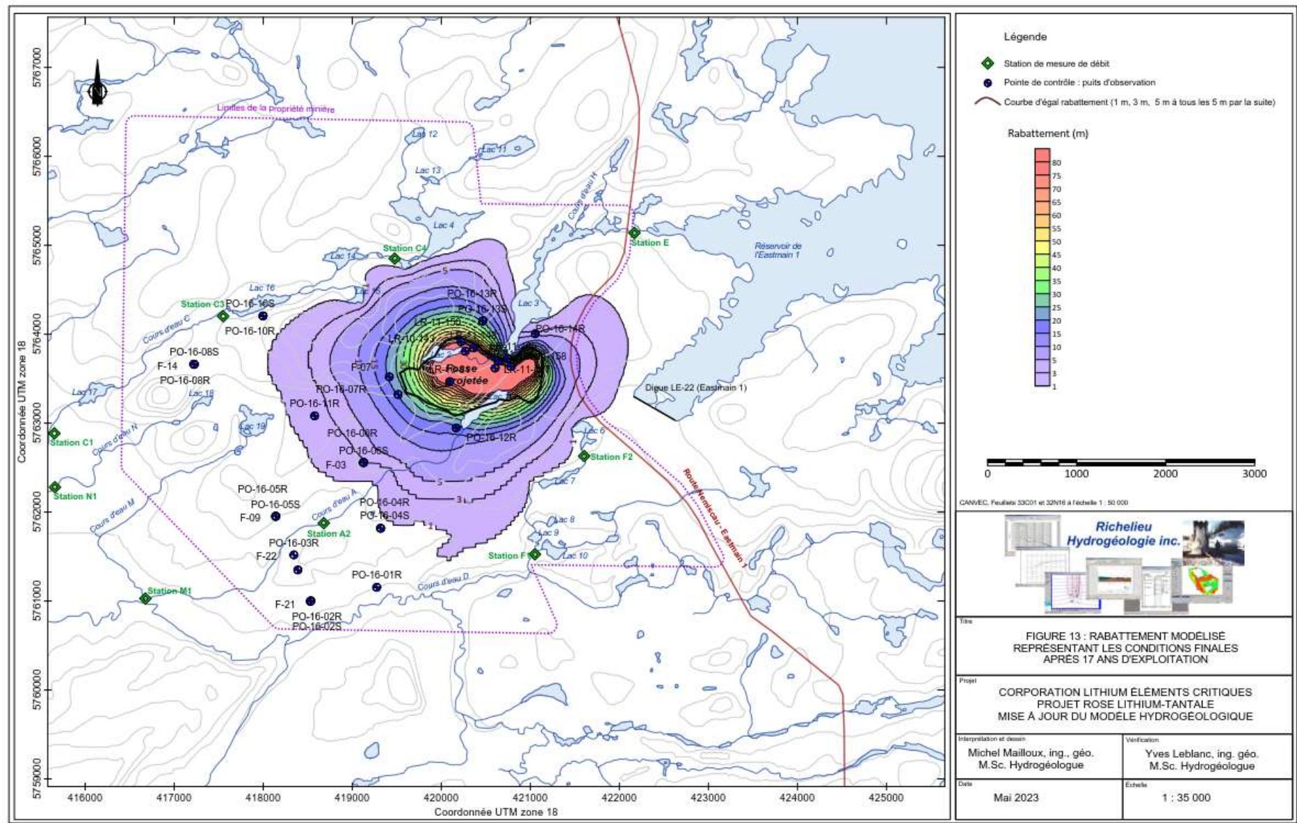
Figure 3 Water table drawdown at the end of 17 years of operation
